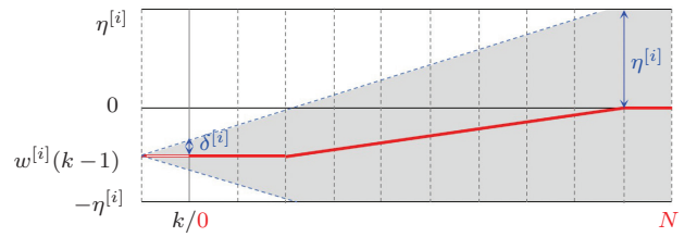
Fig. 1. Prediction of the disturbance. The actual disturbance appears in the shaded area, the red line represents the disturbance prediction \hat{w}_{0:N}(k) over the prediction horizon N .
