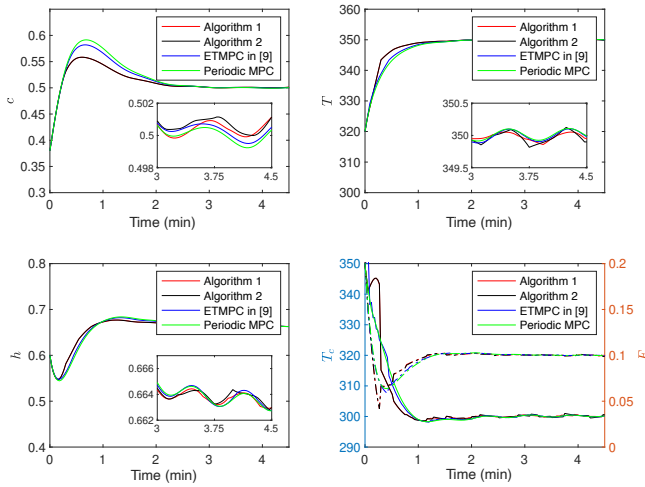
Fig. 2. State evolution and control input under the four MPC schemes. The last subfigure illustrates the coolant liquid temperature T_c (solid) and the outlet flowrate F (dashed).
